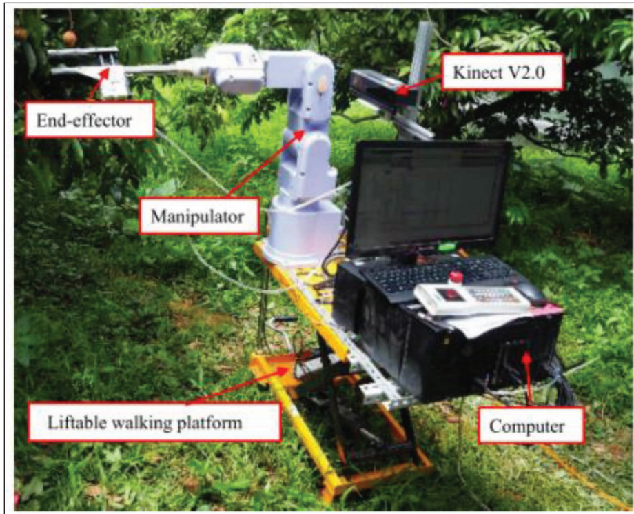
Figure 2. Autonomous fruits and vegetable robotic harvester
